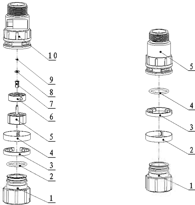
5447001 Flow Meter
