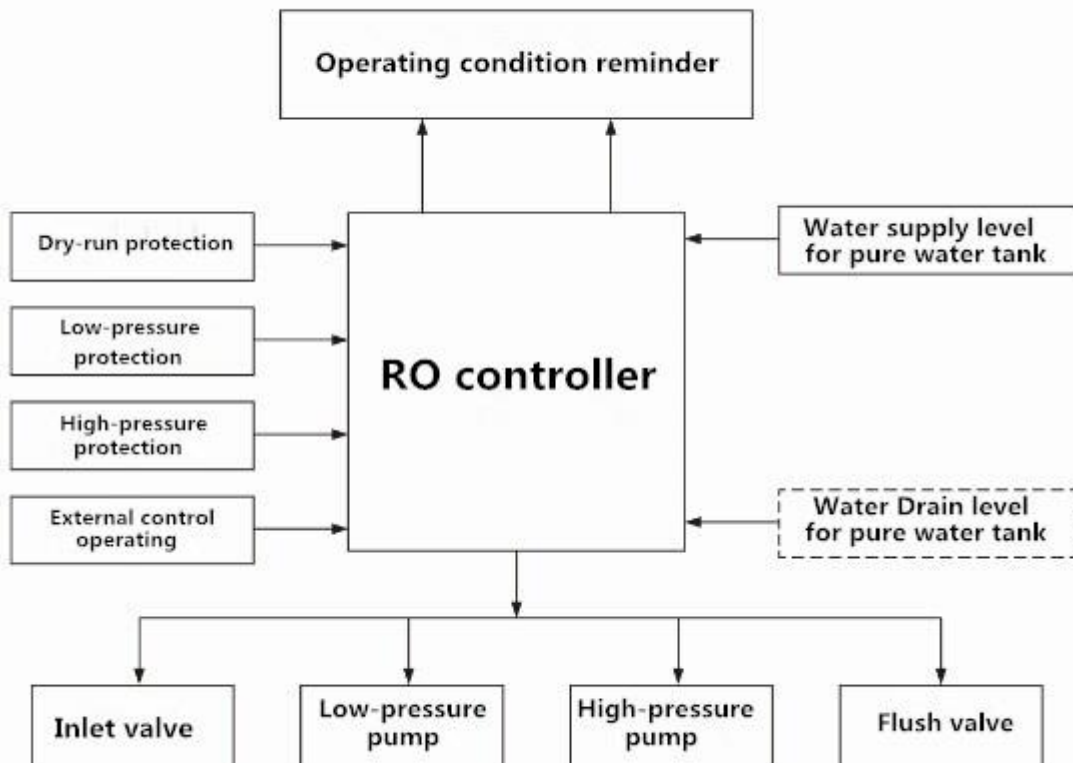
Fig.1 Operating diagram
