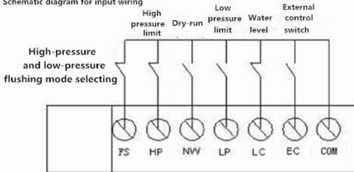
Fig. 5 Schematic diagram for input wiring
